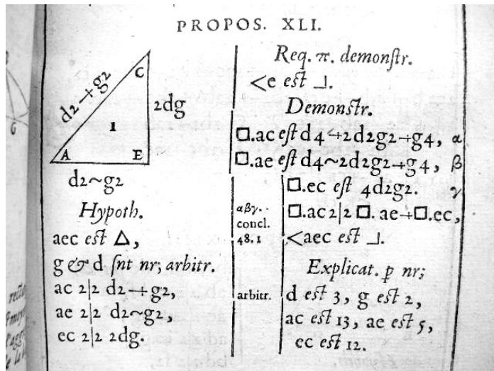
Figure 8. A typical math problem shown by Hérigone in his concise notation.
