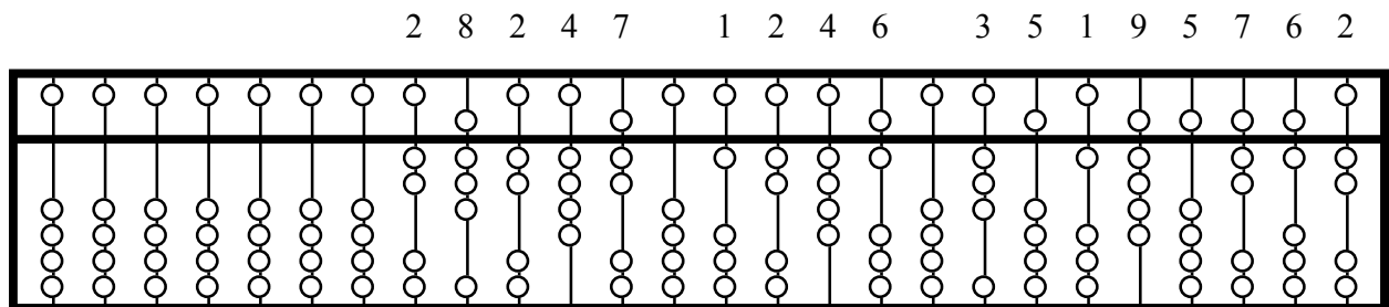
Figure 4. Multiplication on a Japanese soroban abacus
